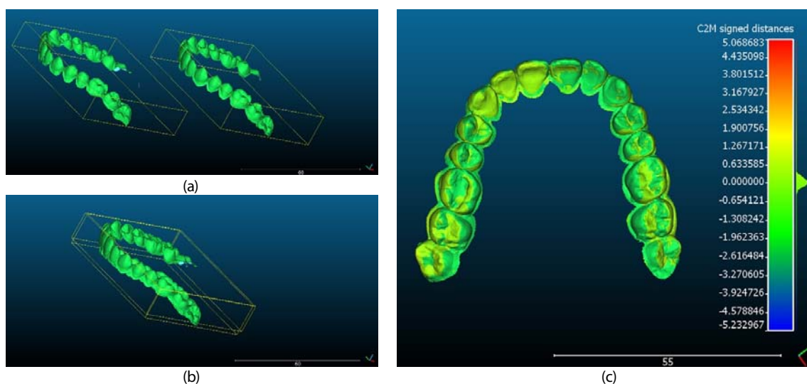
Fig. 4 3D superimposition: (a) The STL format for the scanned conventional impression and IOS; (b) Superimposition of two data; (c) The overlapping of the two data showing colour spectrum of yellow and green indicating minimal Hausdorff distance (HD).
